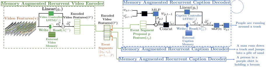
Figure 2: Illustration of our dense captioning model with references to variables in our equations. Encoder components are shown in green and decoder components are shown in blue.
